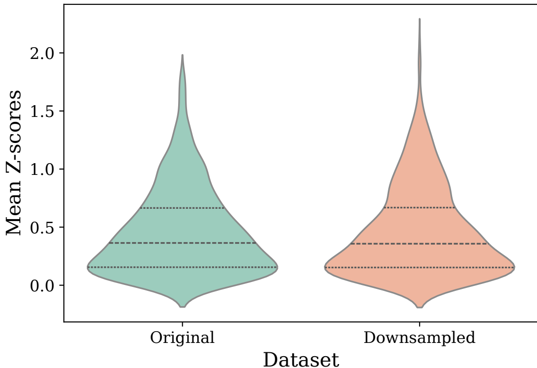
Distribution of Mean Z-scores Original N=100 vs Downsampled N=100k to R=100 \sigma = (0.02, 0.4) v = (0.07, 0.9)
